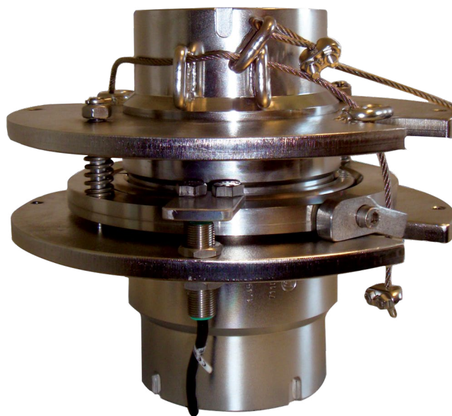
Shown with optional proximity switch
