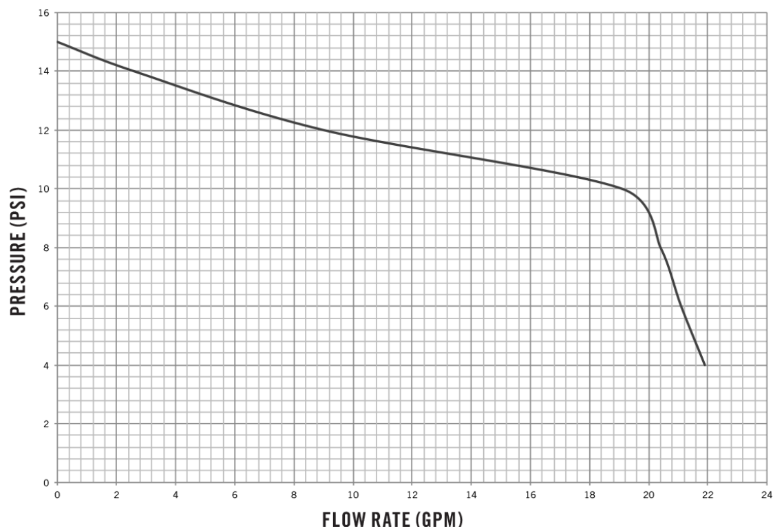
4400 Series Performance Curve
