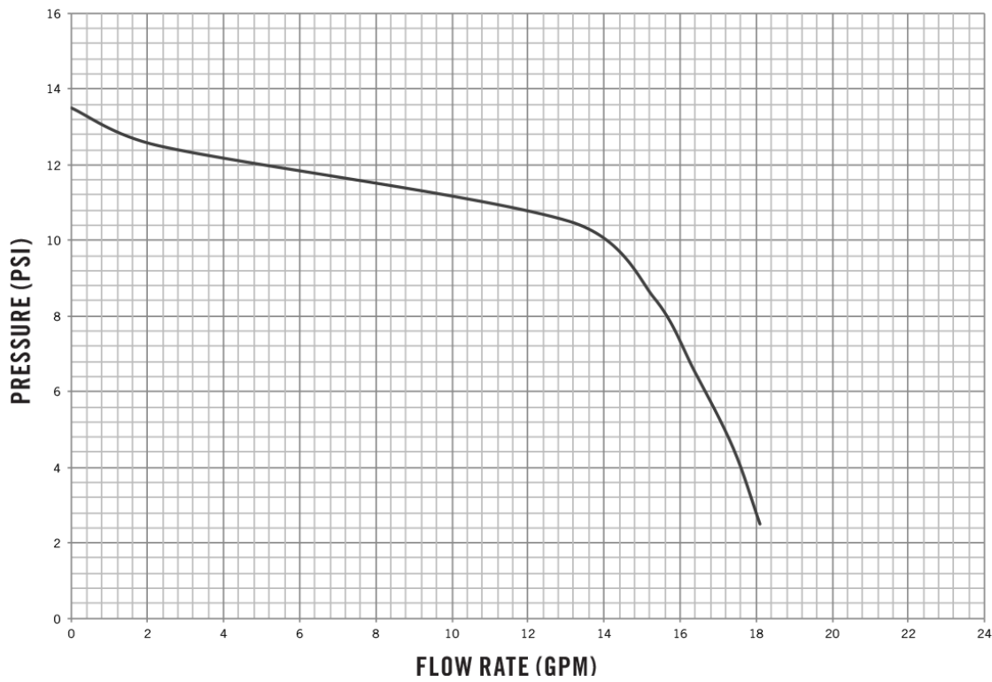
2400 Series Performance Curve
